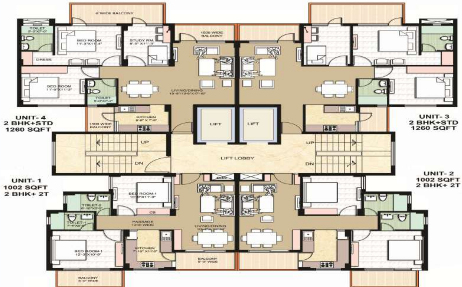
2 BHK 2 TOI. / 2 BHK +STUDY + 2 TOI. TYPICAL FLOOR CLUSTER PLAN
