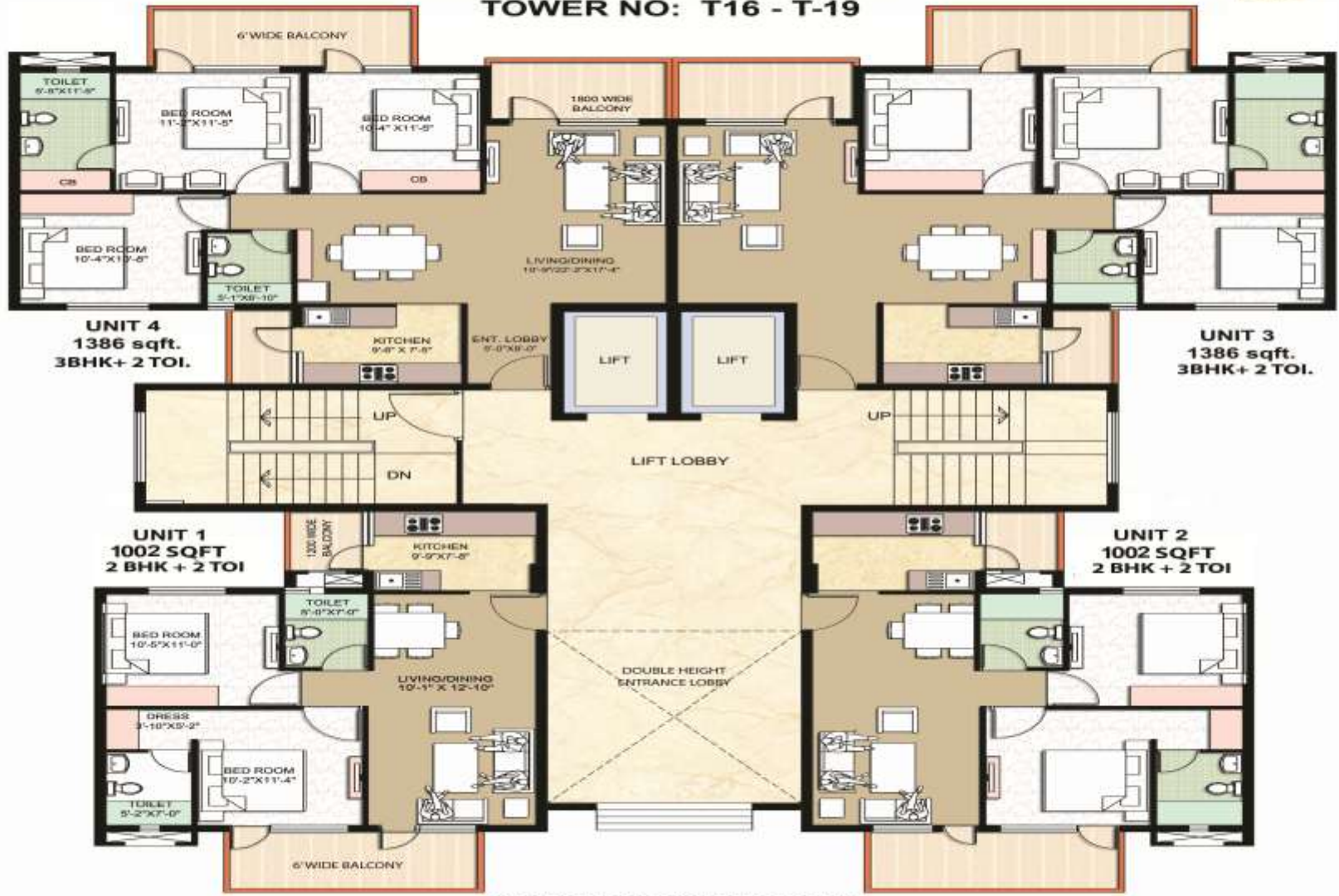
3 BHK + 2 TOI / 2 BHK + 2 TOI. GROUND FLOOR CLUSTER PLAN
